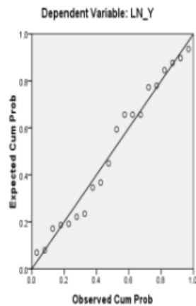
Figure 5. Normal Data Test With Normal P-Plot
